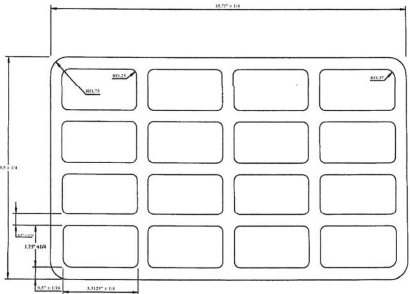
Drawing 1. 9 1/2"x15 1/4" -- 16 Cell Tower Fill Starter Block
