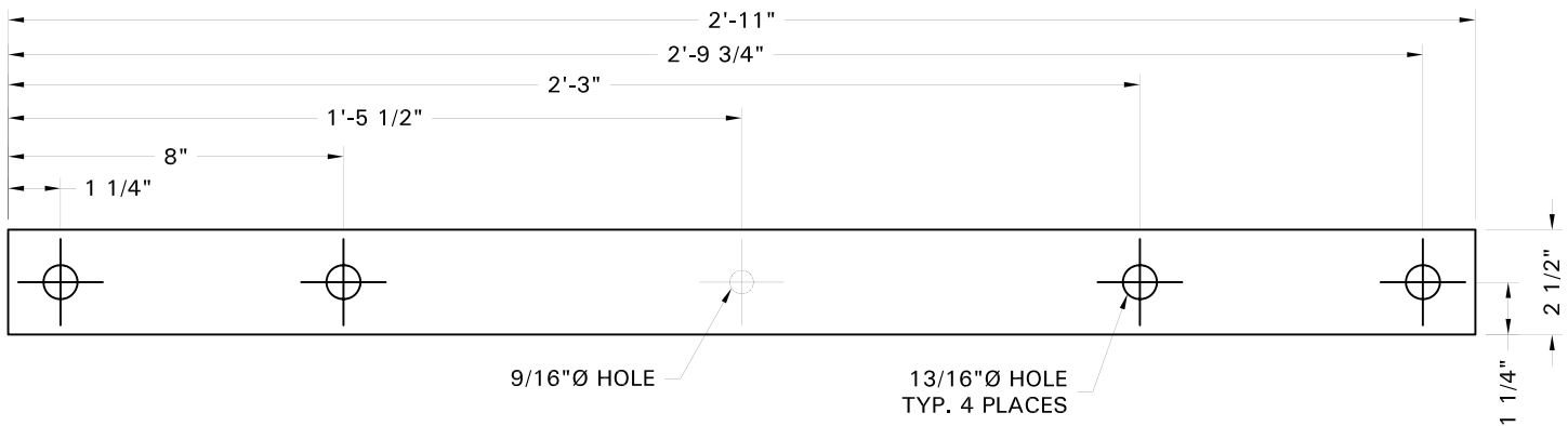
5HS-24 5 HOLE STRAP 2 1/2" x 2'-11" x 3/16" FRP
