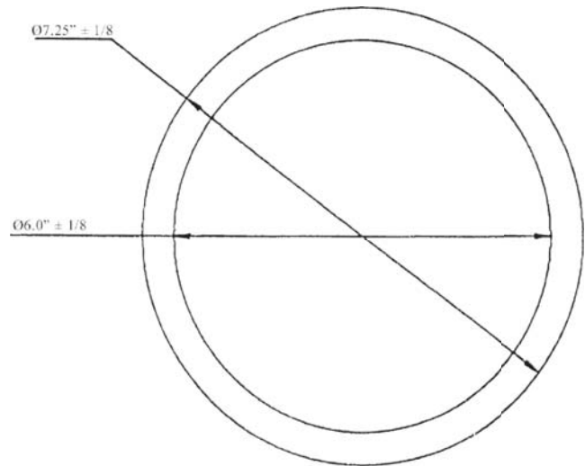
Drawing 3. Spacer Ring
