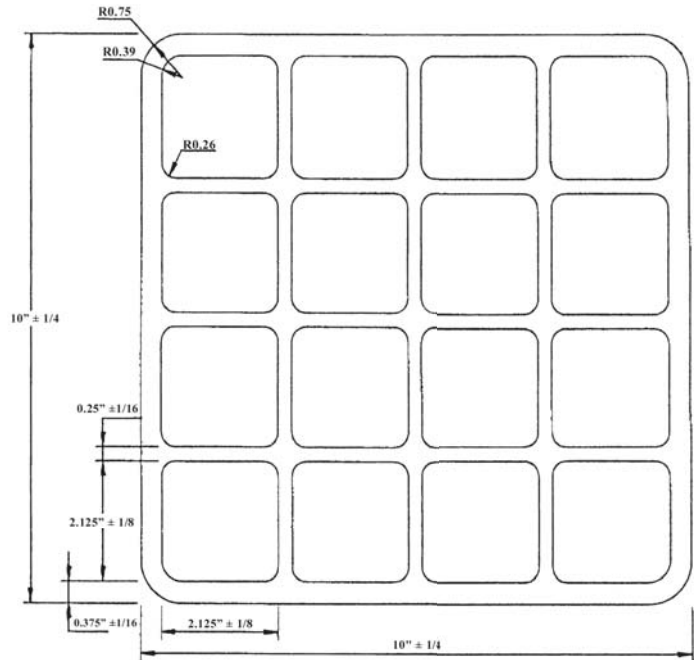
Drawing 2. 10"x10"--16 Cell Tower Fill Block
