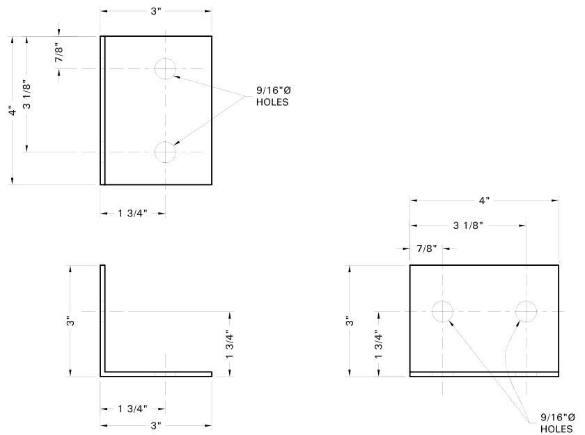
WL-1 WALK WAY "L" BRACKET 3" x 3" x 1/8" x 4" STAINLESS STEEL ANGLE
